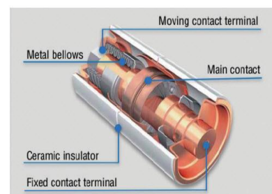
Vacuum Interrupter
