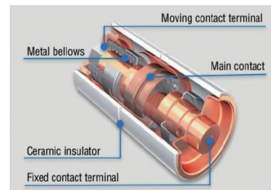
Vacuum Interrupter
