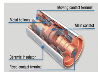
Vacuum Interrupter
